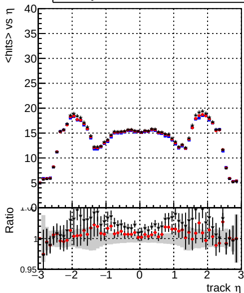
mean hits — DQM_V0001_R000000001_Global_mkFit_baseline — DQM_V0001_R000000001_Global_mkFit_var — DQM_V0001_R000000001_Global_mkFit_coreNoClean
