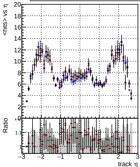
mean hits vs \eta Global_mkFit_baseline Global_mkFit_var Global_mkFit_coreNoClean
