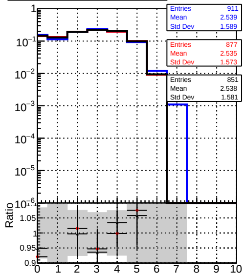
mean hit — DQM_V0001_R000000001_Global_mkFit_baseline — DQM_V0001_R000000001_Global_mkFit_var — DQM_V0001_R000000001_Global_mkFit_coreNoClean
