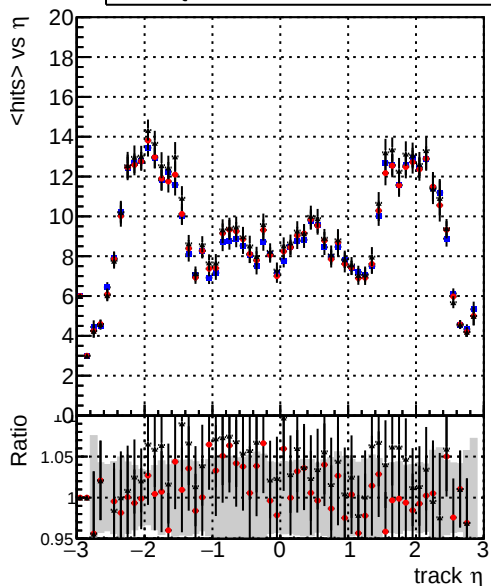
mean hits vs \eta Legend: — DQM_V0001_R000000001_Global_mkFit_baseline (blue) — DQM_V0001_R000000001_Global_mkFit_var (red) — DQM_V0001_R000000001_Global_mkFit_coreNoClean (black)
