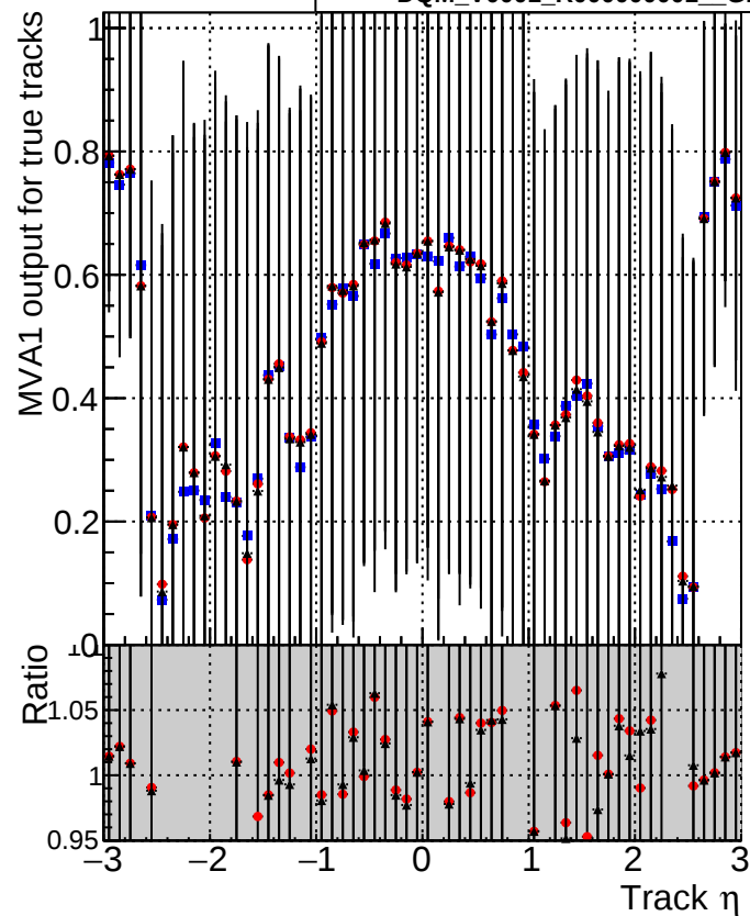
MVA1 of associated tracks (recoToSim) vs. track \eta Legend: ■ DQM_V0001_R000000001_Global_mkFit_baseline ● DQM_V0001_R000000001_Global_mkFit_var ▲ DQM_V0001_R000000001_Global_mkFit_jcoreNoClean
