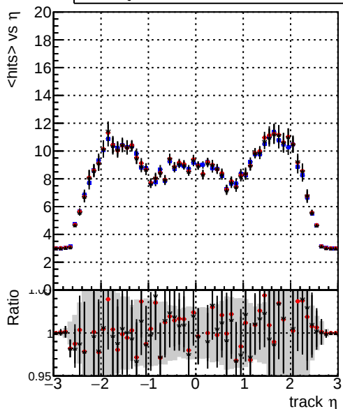
mean hits vs \eta Legend: - DQM_V0001_R000000001_Global_mkFit_baseline (blue line) - DQM_V0001_R000000001_Global_mkFit_var (red line) - DQM_V0001_R000000001_Global_mkFit_coreNoClean (black line)
