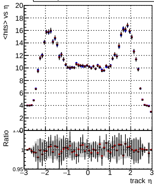
mean hit — DQM_V0001_R000000001_Global_mkFit_baseline — DQM_V0001_R000000001_Global_mkFit_var — DQM_V0001_R000000001_Global_mkFit_jcoreNoClean
