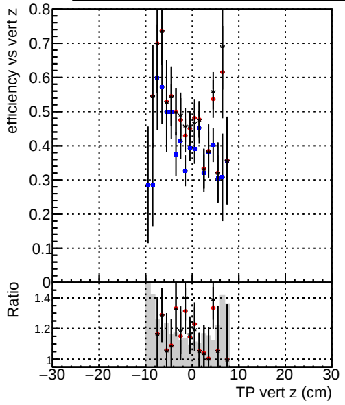
Efficiency vs vertpos Legend: DQM_V0001_R000000001_Global_mkFit_baseline DQM_V0001_R000000001_Global_mkFit_var DQM_V0001_R000000001_Global_mkFit_jcoreNoClean
