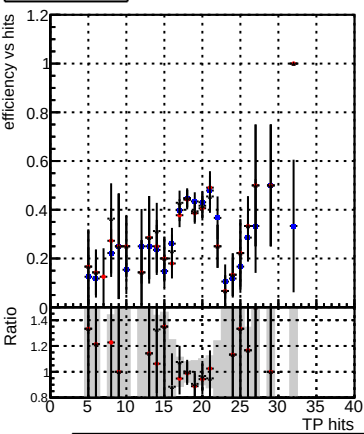
Efficiency vs hit Legend: DQM_V0001_R000000001_Global_mkFit_baseline DQM_V0001_R000000001_Global_mkFit_var DQM_V0001_R000000001_Global_mkFit_jcoreNoClean
