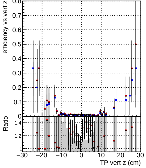
Efficiency vs. sim PV z —●— DQM_V0001_R0000000001_Global_mkFit_baseline —●— DQM_V0001_R0000000001_Global_mkFit_var —●— DQM_V0001_R0000000001_Global_mkFit_coreNoClean
