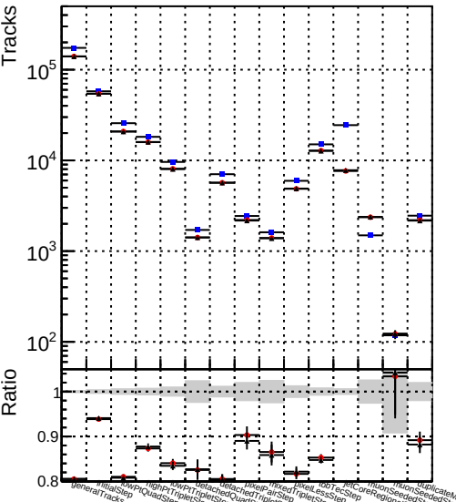
Number DQM_V0001_R0000000001_Global_mkFit_baseline DQM_V0001_R0000000001_Global_mkFit_var DQM_V0001_R0000000001_Global_mkFit_jcureNoClean
