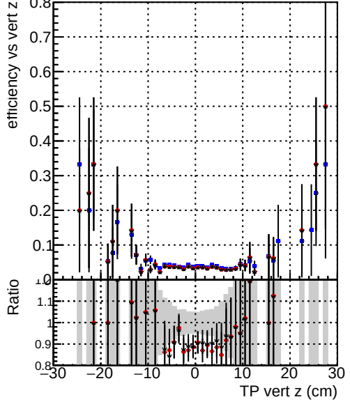
Efficiency vs vert z — DQM_V0001_R0000000001_Global_mkFit_baseline — DQM_V0001_R0000000001_Global_mkFit_var — DQM_V0001_R0000000001_Global_mkFit_coreNoClean
