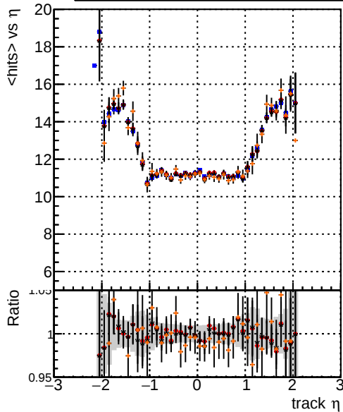
Legend: DQM_V0001_R000000001 Global mkFit baseline, DQM_V0001_R000000001 Global mkFit var, DQM_V0001_R000000001 Global mkFit jcoreNoClean, DQM_V0001_R000000001 Global mkFit jcoreSHits mean hit
