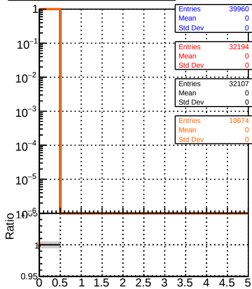
mean hits vs \eta Legend: Blue line: DQM_V0001_R000000001_Global_mkFit_baseline Red line: DQM_V0001_R000000001_Global_mkFit_var Black line: DQM_V0001_R000000001_Global_mkFit_jcoreNoClean Orange line: DQM_V0001_R000000001_Global_mkFit_jcoreSHits
