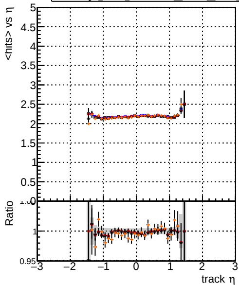
mean hits vs \eta Legend: Blue line: DQM_V0001_R000000001_Global_mkFit_baseline Red line: DQM_V0001_R000000001_Global_mkFit_var Black line: DQM_V0001_R000000001_Global_mkFit_jcoreNoClean Orange line: DQM_V0001_R000000001_Global_mkFit_jcoreSHits
