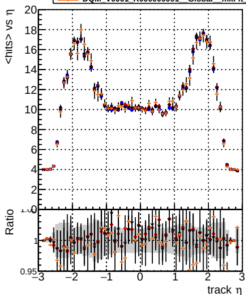
mean hits Legend: DQM_V0001_R000000001 Global mkFit baseline, DQM_V0001_R000000001 Global mkFit var, DQM_V0001_R000000001 Global mkFit jcoreNoClean, DQM_V0001_R000000001 Global mkFit jcoreSHits
