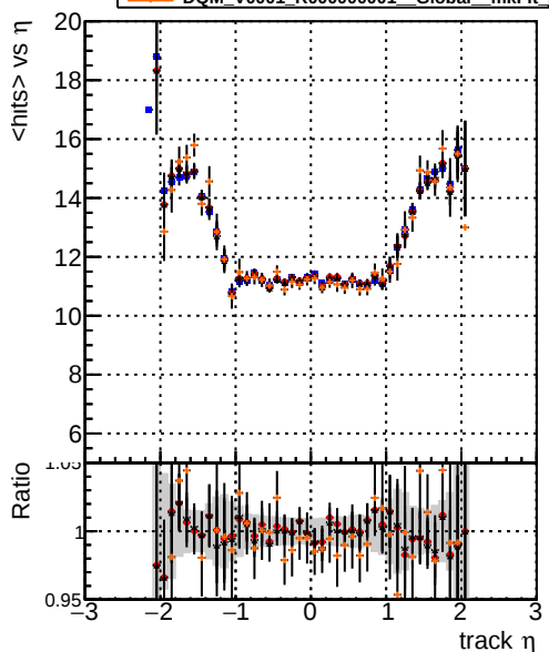
Legend: DQM_V0001_R000000001 Global mkFit baseline, DQM_V0001_R000000001 Global mkFit var, DQM_V0001_R000000001 Global mkFit jcoreNoClean, DQM_V0001_R000000001 Global mkFit jcoreSHits mean hit
