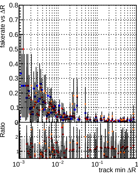
Fake rate vs \Delta R (track, jet) DQM V00001 R00000000001 Global mkFit baseline DQM V00001 R00000000001 Global mkFit var DQM V00001 R00000000001 Global mkFit coreNoClean DQM V00001 R00000000001 Global mkFit coreSHits
