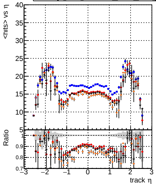
mean hits DQM_V0001_R000000001_Global_mkFit_baseline DQM_V0001_R000000001_Global_mkFit_var DQM_V0001_R000000001_Global_mkFit_coreNoClean DQM_V0001_R000000001_Global_mkFit_coreSHits
