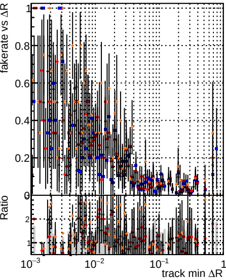
Fake rate vs \Delta R(\text{track, jet}) Legend: DQM V00001 DQM V00001 R00000000001 Global mkFit baseline Global mkFit var Global mkFit coreNoClean Global mkFit coreShifts
