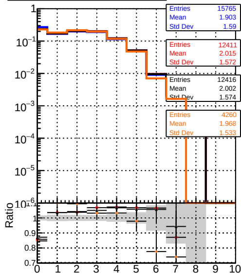
mean hits DQM_V0001_R000000001_Global_mkFit_baseline DQM_V0001_R000000001_Global_mkFit_var DQM_V0001_R000000001_Global_mkFit_jcoreNoClean DQM_V0001_R000000001_Global_mkFit_jcoreSHits
