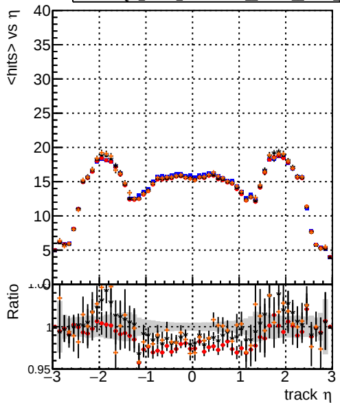
Legend for mean hits vs \eta : Blue line: DQM_V0001_R000000001_Global_mkFit_baseline Red line: DQM_V0001_R000000001_Global_mkFit_var Black line: DQM_V0001_R000000001_Global_mkFit_jcNoClean Orange line: DQM_V0001_R000000001_Global_mkFit_jcNoSHits
