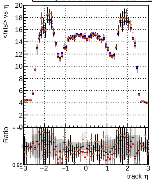
mean hits DQM_V0001_R0000000001 Global mkFit baseline DQM_V0001_R0000000001 Global mkFit var DQM_V0001_R0000000001 Global mkFit jcoreNoClean DQM_V0001_R0000000001 Global mkFit jcoreSHits
