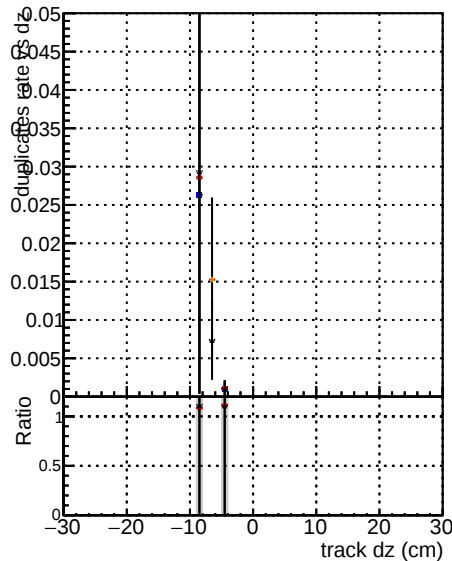
mkFit baseline var mkFit var coreNoClean mkFit coreNoClean coreShits mkFit coreShits
