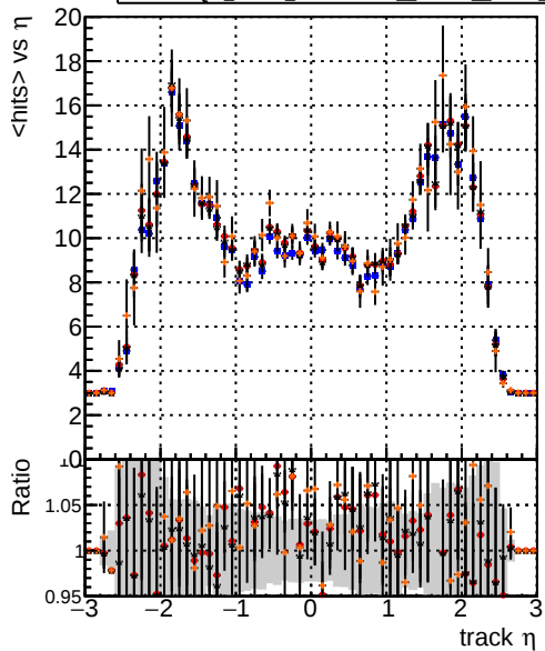
mean hits Legend: DQM_V0001_R000000001_Global_mkFit_baseline (blue line) DQM_V0001_R000000001_Global_mkFit_var (red line) DQM_V0001_R000000001_Global_mkFit_jcoreNoClean (black line) DQM_V0001_R000000001_Global_mkFit_jcoreSHits (orange line)
