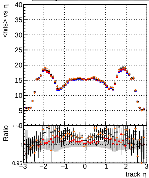
mean hits Legend: DOM_V0001_R000000001_Global_mkFit_baseline DOM_V0001_R000000001_Global_mkFit_var DOM_V0001_R000000001_Global_mkFit_jcoreNoClean DOM_V0001_R000000001_Global_mkFit_jcoreSHits
