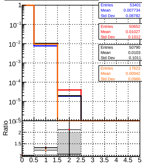
mean hits Legend: DOM_V0001_R000000001_Global_mkFit_baseline DOM_V0001_R000000001_Global_mkFit_var DOM_V0001_R000000001_Global_mkFit_jcoreNoClean DOM_V0001_R000000001_Global_mkFit_jcoreSHits
