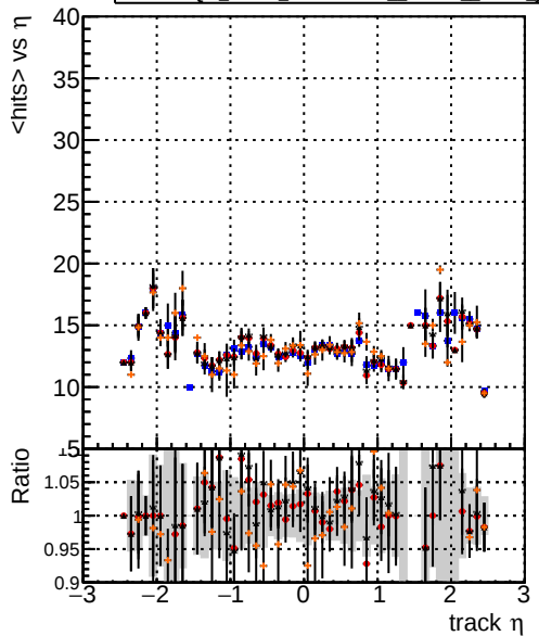
mean hits vs \eta Legend: DQM_V0001_R000000001_Global_mkFit_baseline (blue), DQM_V0001_R000000001_Global_mkFit_var (red), DQM_V0001_R000000001_Global_mkFit_jcoreNoClean (orange), DQM_V0001_R000000001_Global_mkFit_jcoreSHits (black)
