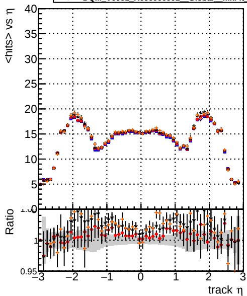
mean hits DQM_V0001_R000000001_Global_mkFit_baseline DQM_V0001_R000000001_Global_mkFit_var DQM_V0001_R000000001_Global_mkFit_jcoreNoClean DQM_V0001_R000000001_Global_mkFit_jcoreSHits
