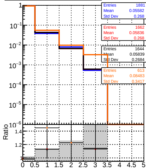
mean hits DQM_V0001_R000000001 Global_mkFit_baseline DQM_V0001_R000000001 Global_mkFit_var DQM_V0001_R000000001 Global_mkFit_coreNoClean DQM_V0001_R000000001 Global_mkFit_coreSHits
