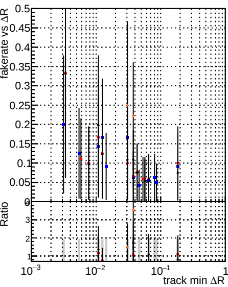
Fake rate vs \Delta R(\text{track, jet}) | Global mktFit baseline | Global mktFit var | Global mktFit coreNoClean | Global mktFit coreShits
