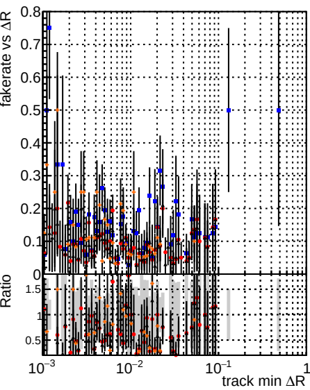
Fake rate vs \Delta R(\text{track}, \text{jet}) Legend: DQM V00001 Global mkFit baseline Global mkFit var Global mkFit coreNoClean Global mkFit coreShifts
