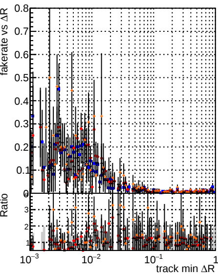
Fake rate vs \Delta R(\text{track, jet}) Legend: Global, mkFit, baseline, Global, mkFit, var, Global, NoClean, Global, coreShifts
