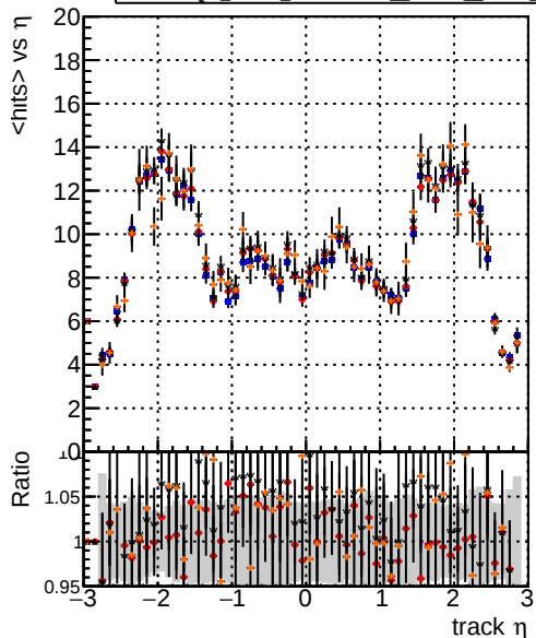
mean hits DQM_V0001_R000000001 Global mkFit baseline DQM_V0001_R000000001 Global mkFit var DQM_V0001_R000000001 Global mkFit jcoreNoClean DQM_V0001_R000000001 Global mkFit jcoreSHits
