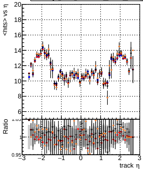
mean hits DQM_V0001_R000000001_Global_mkFit_baseline DQM_V0001_R000000001_Global_mkFit_var DQM_V0001_R000000001_Global_mkFit_coreNoClean DQM_V0001_R000000001_Global_mkFit_icoreSHits
