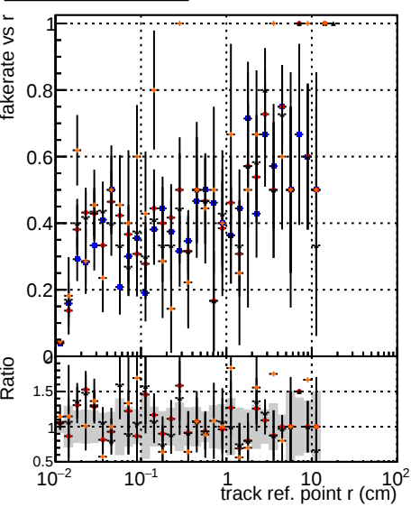
Fake rate vs v Legend: Global mkFit baseline (black) Global mkFit var (blue) Global mkFit coreNoClean (red) Global mkFit coreShits (orange)
