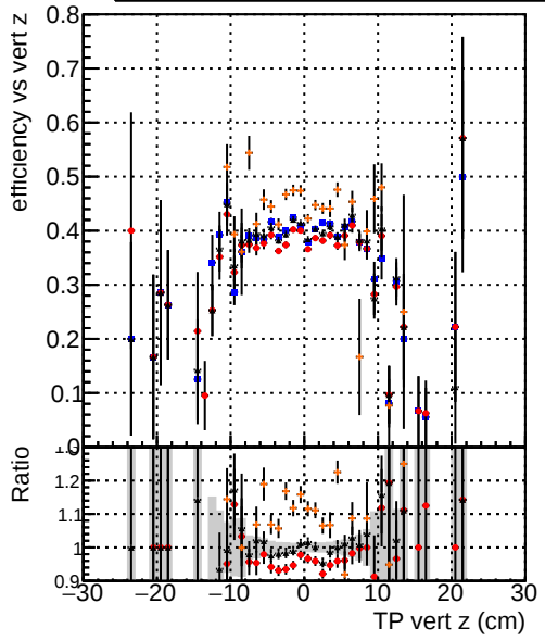
Efficiency vs vert z —●— DQM_V0001_R000000001 Global_mkFit_baseline —●— DQM_V0001_R000000001 Global_mkFit_var —●— DQM_V0001_R000000001 Global_mkFit_coreNoClean —●— DQM_V0001_R000000001 Global_mkFit_coreSHits
