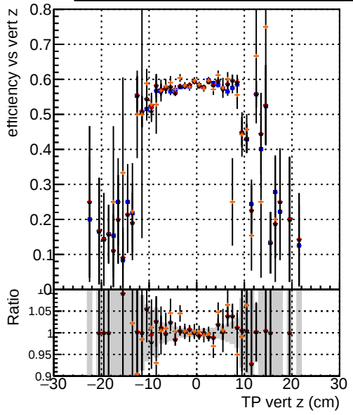
Efficiency vs vert z —●— DQM_V0001_R0000000001 Global_mkFit_baseline —●— DQM_V0001_R0000000001 Global_mkFit_var —●— DQM_V0001_R0000000001 Global_mkFit_jcoreNoClean —●— DQM_V0001_R0000000001 Global_mkFit_jcoreSHits
