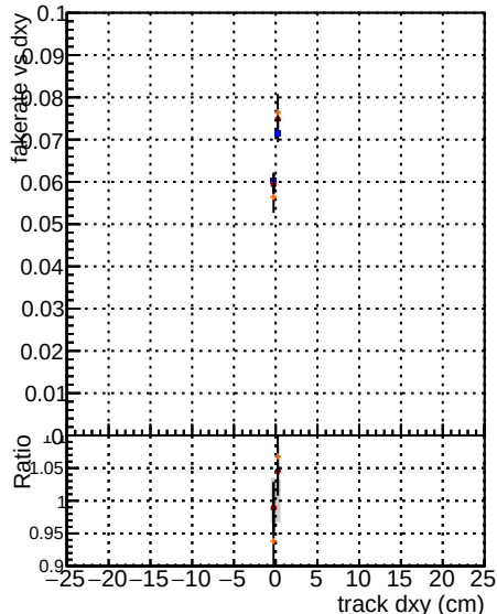
Fake rate vs d Global mkFit baseline Var DOM V0001 B00000000001 Global mkFit baseline DOM V0001 B00000000001 Global mkFit Var DOM V0001 R00000000001 Global mkFit baseline DOM V0001 R00000000001 Global mkFit Var CoreNoClean CoreSHits
