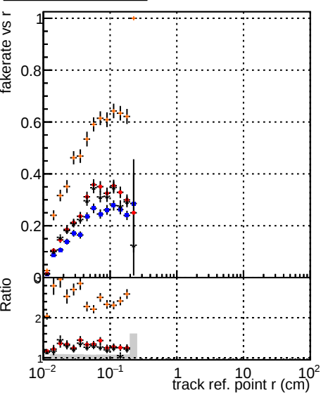
Fake rate vs v Series Color Shape Global Black Line Global mkFit Blue Circle Global mkFit var Red Circle Global mkFit var NoClean Orange Circle Global mkFit var NoClean SHits Purple Circle
