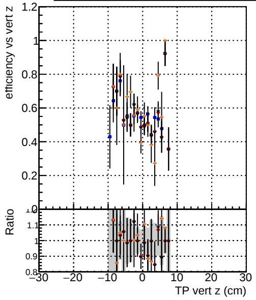
Efficiency vs vertpos —●— DQM_V0001_R0000000001 Global_mkFit_baseline —●— DQM_V0001_R0000000001 Global_mkFit_var —●— DQM_V0001_R0000000001 Global_mkFit_jcoreNoClean —●— DQM_V0001_R0000000001 Global_mkFit_jcoreSHits
