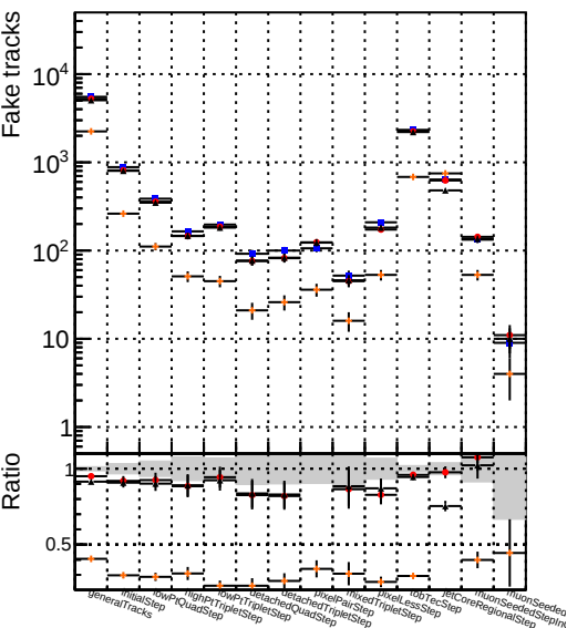
Number Symbol QID QID QID QID QID QID ▲ DQM V0001 R000000001 Global mkFit coreNoClean ● DQM V0001 R000000001 Global mkFit coreSHits
