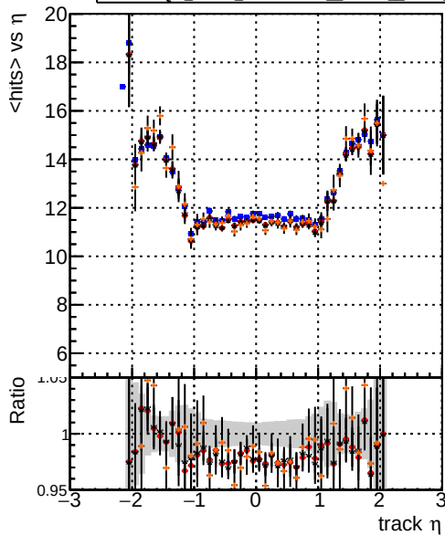
Legend for mean hits vs \eta : DQM_V0001_R000000001_Global_mkFit_baseline DQM_V0001_R000000001_Global_mkFit_var DQM_V0001_R000000001_Global_mkFit_jcoreNoClean DQM_V0001_R000000001_Global_mkFit_jcoreSHits
