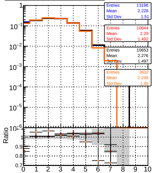
Legend for mean hits vs \eta : DQM_V0001_R000000001_Global_mkFit_baseline DQM_V0001_R000000001_Global_mkFit_var DQM_V0001_R000000001_Global_mkFit_jcoreNoClean DQM_V0001_R000000001_Global_mkFit_jcoreSHits
