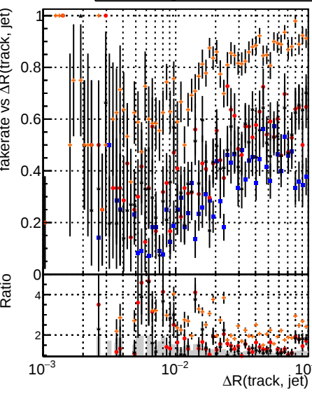
Fake rate vs \Delta R(\text{track, jet}) Legend: Global mktFit baseline var coreNoClean coreSHits
