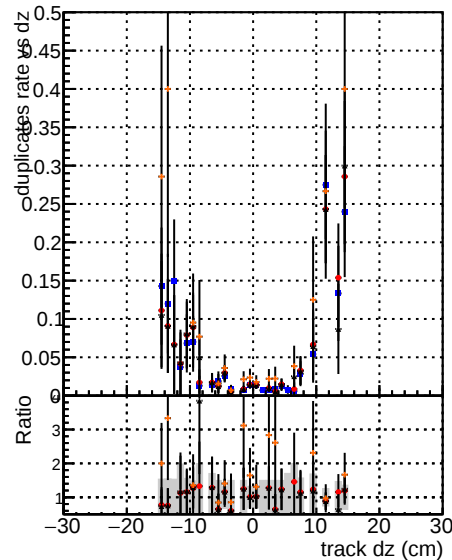
mkFit baseline var coreNoClean coreSHits mkFit ✓ ✓ ✓ ✓ X baseline ✓ ✓ ✓ ✓ X var ✓ ✓ ✓ ✓ X coreNoClean ✓ ✓ ✓ ✓ X coreSHits ✓ ✓ ✓ ✓ X
