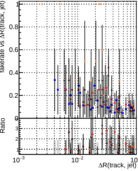
Fake rate vs \Delta R(\text{track, jet}) DQM V00001 Global mkFit baseline Global mkFit var Global mkFit coreNoClean Global mkFit coreSHits
