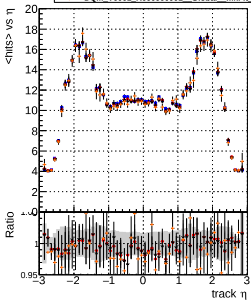
mean hits vs \eta Legend: DQM_V0001_R000000001_Global_mkFit_baseline DQM_V0001_R000000001_Global_mkFit_var DQM_V0001_R000000001_Global_mkFit_coreNoClean DQM_V0001_R000000001_Global_mkFit_coreSHits
