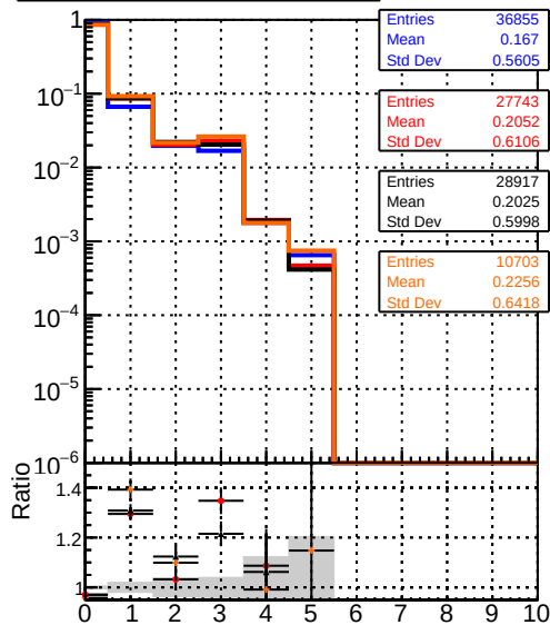
mean hits Legend: DQM_V0001_R000000001 Global mkFit baseline, DQM_V0001_R000000001 Global mkFit var, DQM_V0001_R000000001 Global mkFit jcoreNoClean, DQM_V0001_R000000001 Global mkFit jcoreSHits
