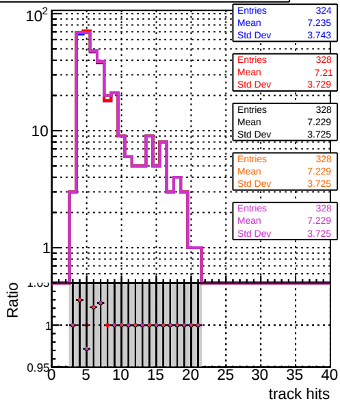
Legend: DOM V0001 R0000000001 Global CMSSW prd008, DOM V0001 R0000000001 Global CMSSW hptt05, DOM V0001 R0000000001 Global CMSSW hptt03, DOM V0001 R0000000001 Global CMSSW hptt01
