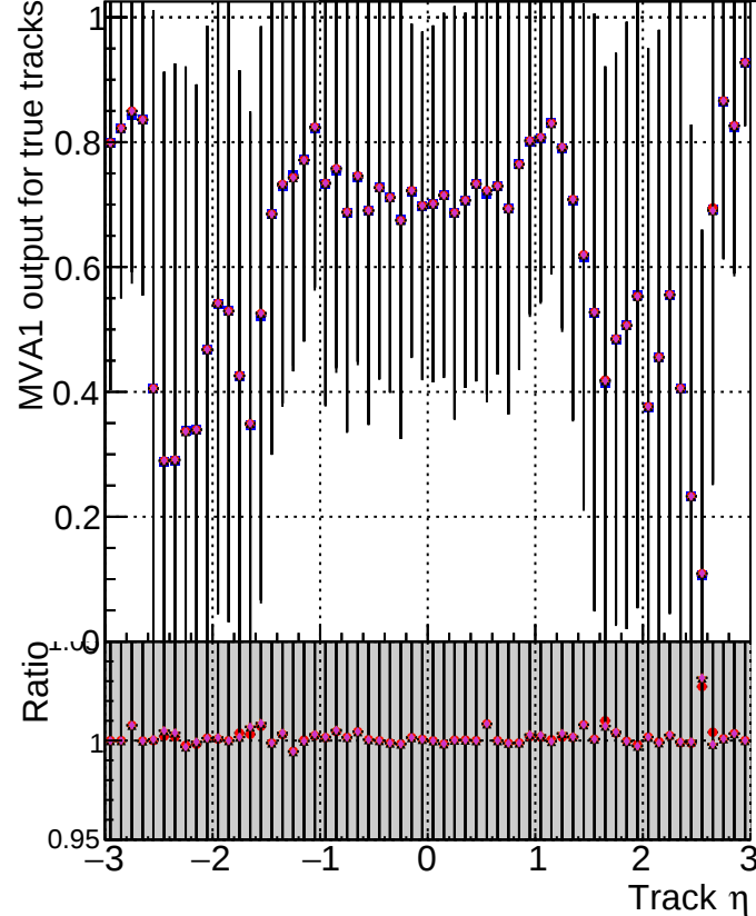
MVA1 of associated tracks (recoToSim) vs. track \eta Legend Model Region Global CMSSW Model Blue square DQM V0001 R000000001 Global CMSSW orig Red circle DQM V0001 R000000001 Global CMSSW hptt08 Black triangle DQM V0001 R000000001 Global CMSSW hptt05 Orange diamond DQM V0001 R000000001 Global CMSSW hptt03 Purple star DQM V0001 R000000001 Global CMSSW hptt01
