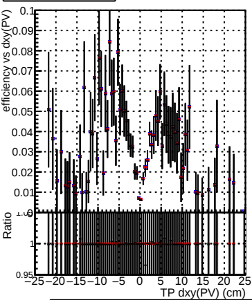
Efficiency vs Dxy(PV) Legend: DQM_V0001_R000000001_Global_CMSSW_orig DQM_V0001_R000000001_Global_CMSSW_dt08 DQM_V0001_R000000001_Global_CMSSW_dt05
