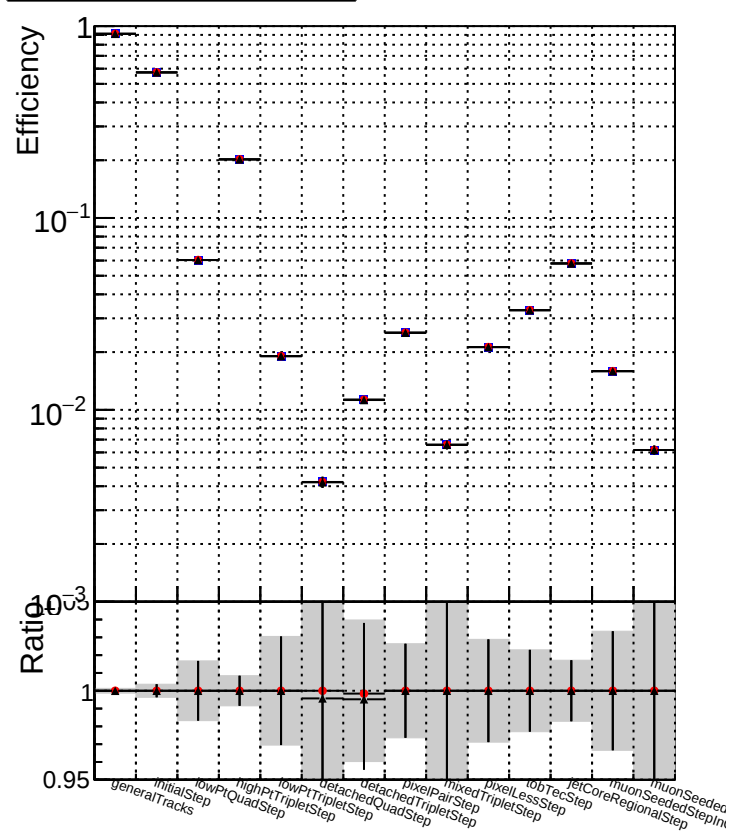
Duplicates rate vs collection Legend: DQM_V0001_R000000001_Global_CMSSW_orig DQM_V0001_R000000001_Global_CMSSW_dt08 DQM_V0001_R000000001_Global_CMSSW_dt05
